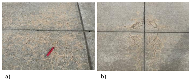
a) b) Figure 1 a) and b) existing durability cracking and potential alkali-silica reaction distresses observed on the existing concrete
