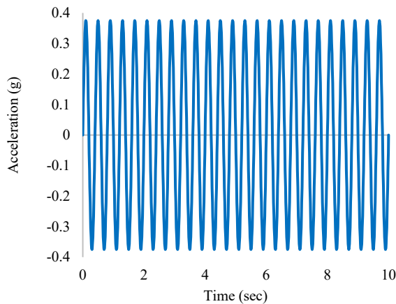
Figure 6. Input motion with amplitude of 0.375g
