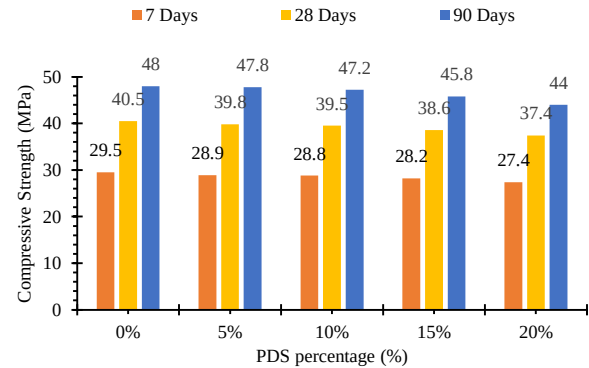
Figure 4. Compressive strength of concrete samples with different percentages of PDS replacement alongside 20% fly ash at different ages
